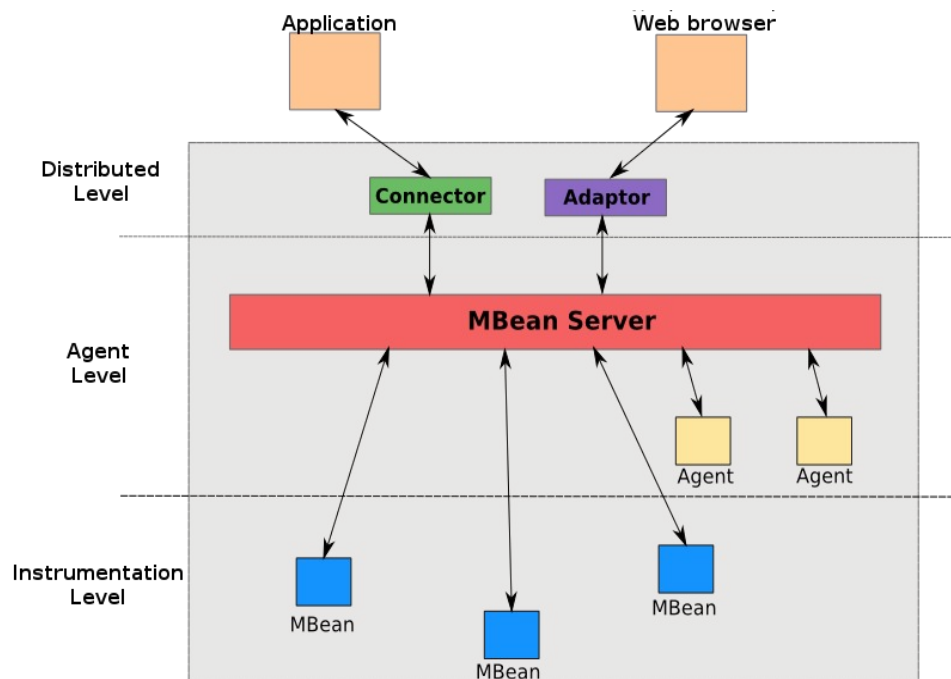
Illustration 1: Architecture JMX
